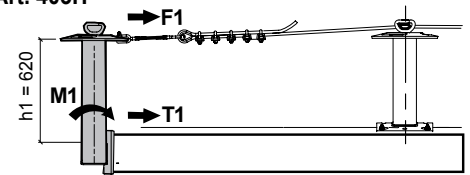
Art. 403H
